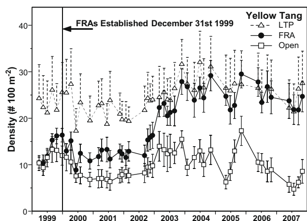
Fig. 3. Mean yellow tang density trends ( \pm SE) at West Hawaii monitoring sites. Data exclude young-of-year. LTP sites ( n = 5 ) were closed to aquarium collecting since at least 1991. FRA sites ( n = 9 ) are Fish Replenishment Areas, i.e. were open to fishers prior to establishment of the FRA network. Open sites ( n = 9 ) were open to fishers throughout the study. Monitoring stations were located in yellow tang juvenile habitat, thus densities reflect sub-adult fish. Only upper SE bars shown for LTP sites.
